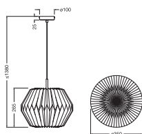
DECOR PAPER LANTERN GEM PEND E27
