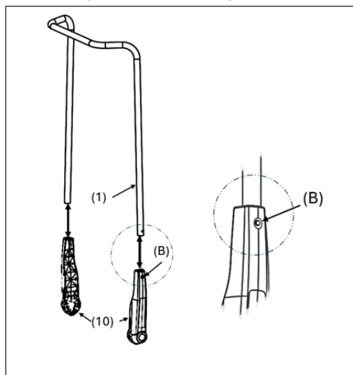
Fig. 2: Fitting the handle fittings
