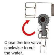
④ Close the three-way valve
